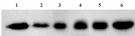
Fig 4. Representative Western-blot analysis of cytoplasmic proteins demonstrating the effect of \alpha -pinene on LPS-mediated degradation of I \kappa B \alpha in THP-1 cells. Lane 1: control; Lane 2: LPS 1 mg/L for 30 min; Lane 3-6: \alpha -pinene 1, 10, and 100 mg/L or TLCK 50 \mu mol/L for 30 min before the addition of LPS for 30 min, respectively. Results are representatives of three independent experiments.
