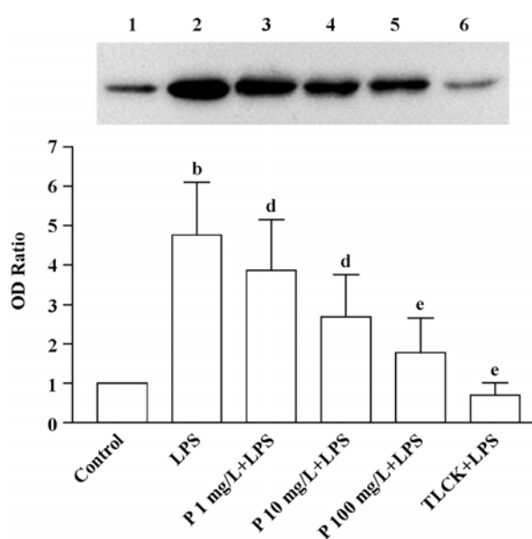
Fig 3. Representative Western-blot analysis of nuclear proteins demonstrating the effect of \alpha -pinene on LPS-mediated nuclear translocation of the NF- \kappa B/p65 in THP-1 cells. Lane 1: control; Lane 2: LPS 1 mg/L for 30 min; Lane 3-6: \alpha -pinene 1, 10, and 100 mg/L or TLCK 50 \mu mol/L for 30 min before the addition of LPS for 30 min, respectively. n=3 . Mean \pm SD. b P<0.05 vs control. d P>0.05 , e P<0.05 vs LPS.
